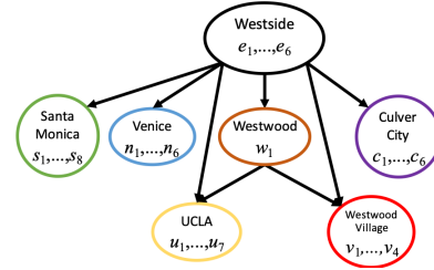
Figure 19: Specifying conditional independence relationships using a directed acyclic graph. The relationship between a node and its parent requires a conditional space.
