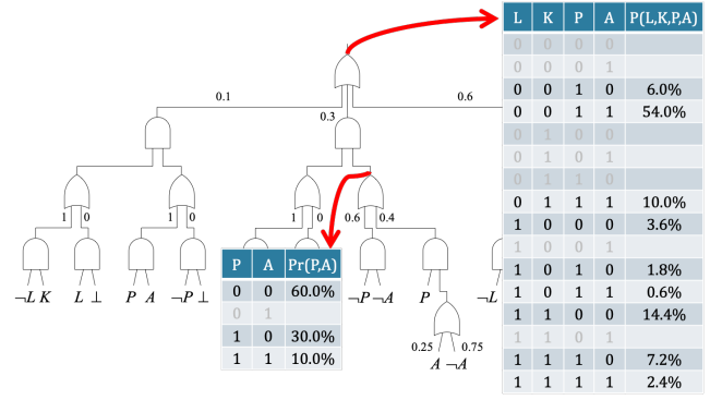
Figure 14: The compositional distributions of a PSDD circuit.
