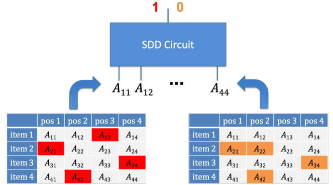
Figure 17: Encoding rankings (total orderings) using SDDs. The red variable assignment (left) encodes a valid ranking. The orange variable assignment (right) does not encode a valid ranking (e.g., item 2 appears in two positions).
