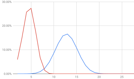
Figure 29: Robustness level vs. proportion of instances for two neural networks with similar accuracies. Net 1 is plotted in blue (right) and Net 2 in red (left).
