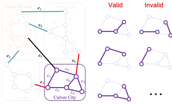
Figure 20: Illustrating the notion of a conditional space. The valid routes inside Culver City are a function of the Westside crossings we use to enter and exit the city.
